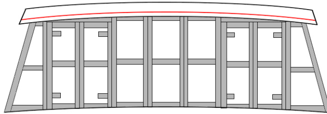
Bulkhead No. 11
